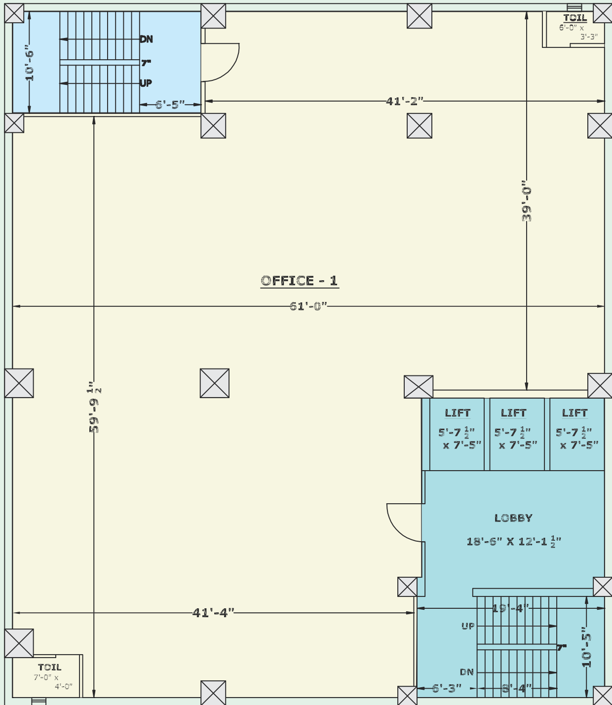
TYPICAL 7TH TO 14TH FLOOR PLAN
